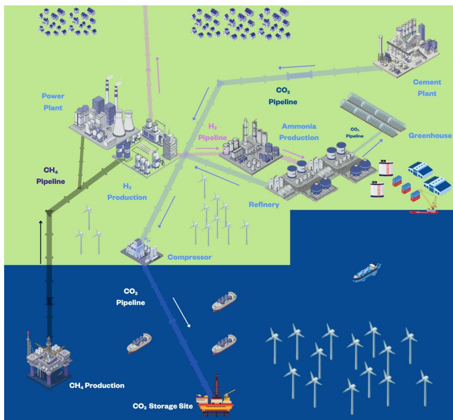
Figure 5: Illustrative example of an industrial carbon management value chain 48
